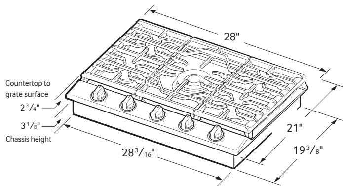
Cooktop Dimensions
