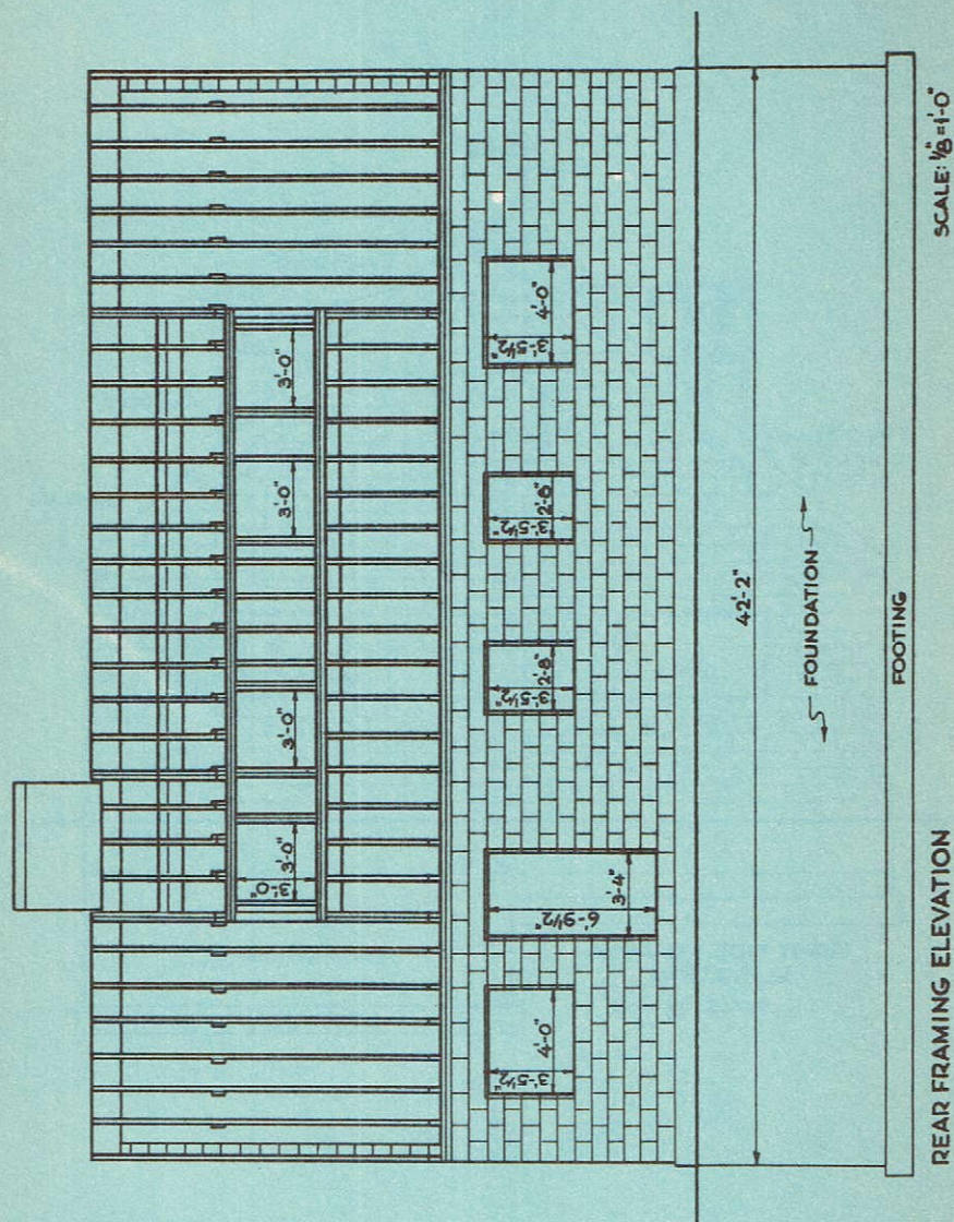
Rear Framing Elevation of the Colonial House
