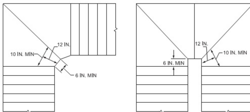
Figure R311.7.5.2.1(1)
