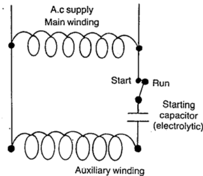
Figure 2. Capacitor motor with a starting capacitor (electrolytic).
