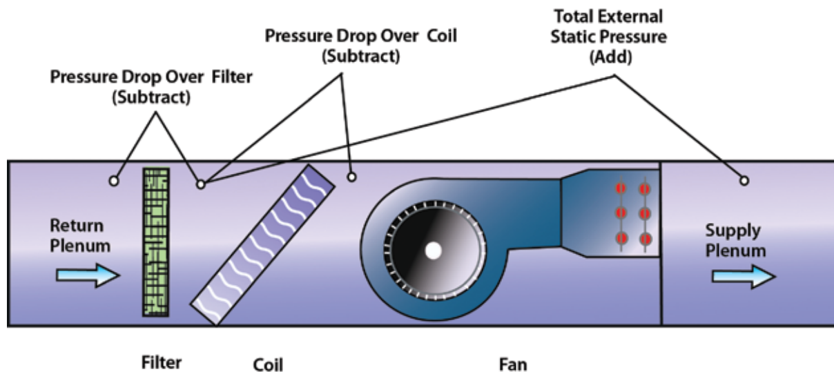
Figure 1 Horizontal air-handler static pressure test locations.
