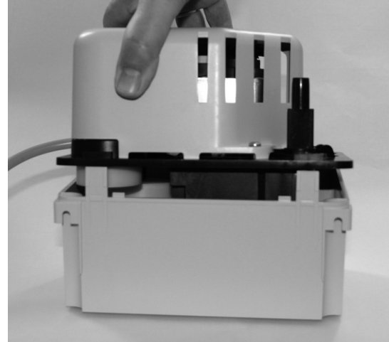
Condensate Inlet on right
