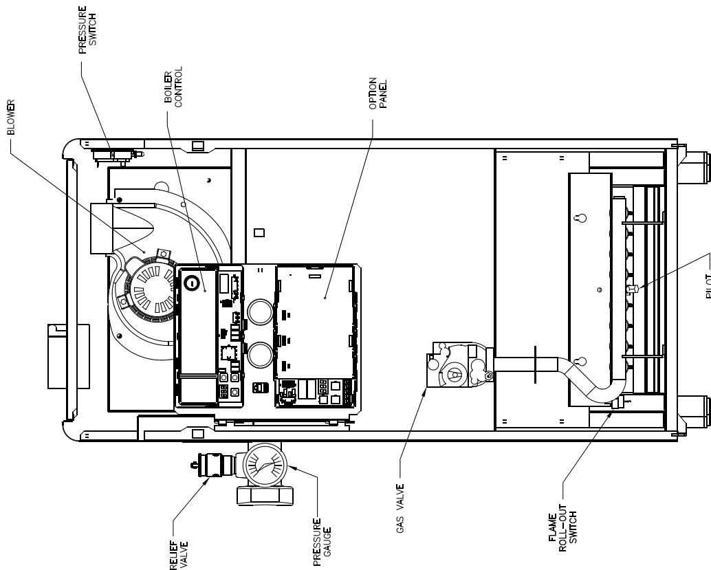
FRONT VIEW AIR BOX, AIR BOX COVER, FRONT DOOR AND FRONT COVER REMOVED
