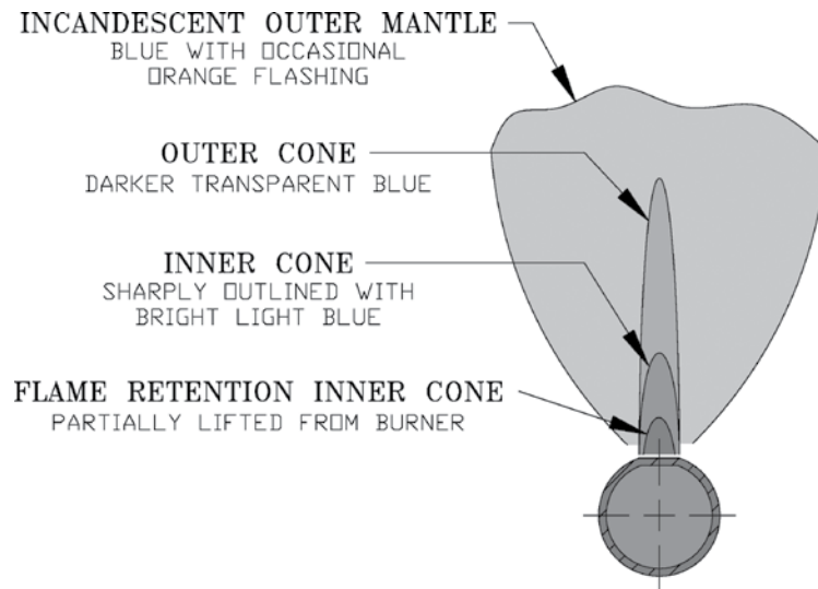
Figure 5: Main Burner Flame
