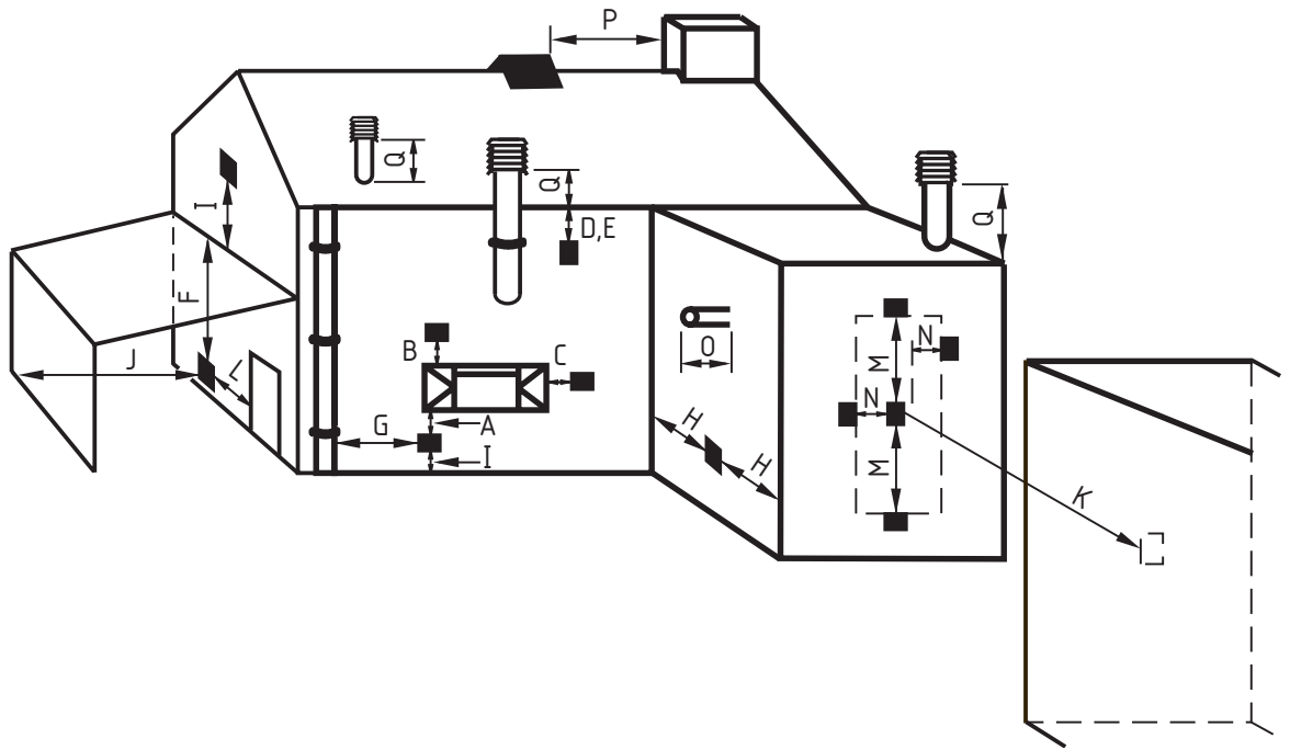
Figure C.1 — Flue terminal positions
