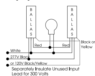
Wiring Diagram 22
