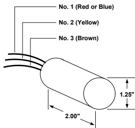
Ref. Drawing 24
