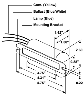
Ref. Drawing 31
