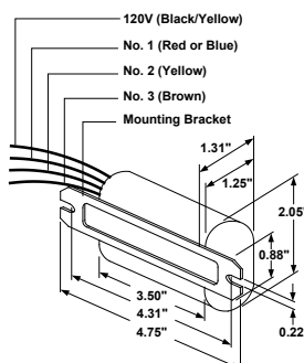
Ref. Drawing 28
