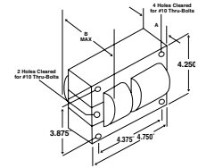
REFERENCE DRAWING PC2
