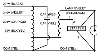
Wiring Diagram 10
