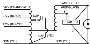
Wiring Diagram 9
