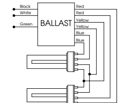
DIAGRAM 20 Series lamp operation
