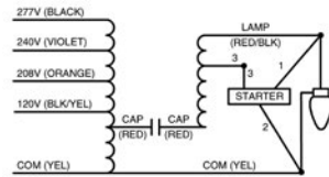
Wiring Diagram 1
