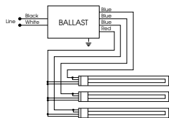
DIAGRAM 14 Parallel lamp operation
