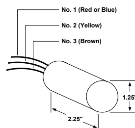
Ref. Drawing 26
