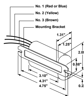
Ref. Drawing 29
