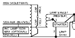
Wiring Diagram 8
