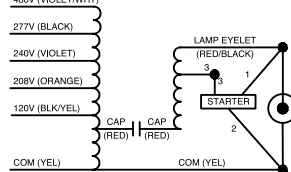
Wiring Diagram 7
