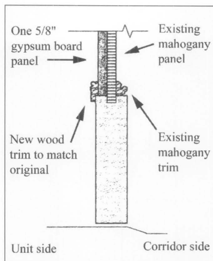
Figure 8. Section of lower wood panel with gypsum board reinforcement. Drawing: Garek Stefanowski, Pappageorge/Haymes.
