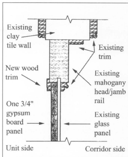
Figure 7. Section of Fisher Building door modified to improve glass panel fire rating. Drawing: Garek Stefanowski, Pappageorge/Haymes.
