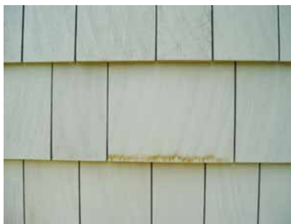
Figure 15. Single coat of solid-color stain. Note the extractives bleed.
