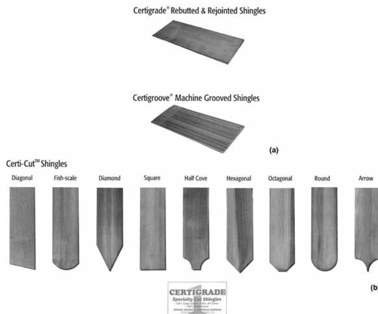
Figure 6. Specialty cut shingles: a, rebutted and rejoined shingles, machine grooved shingles; b, butt-end design. Used with permission from Cedar Shake and Shingle Bureau Exterior and Interior Wall Manual .
