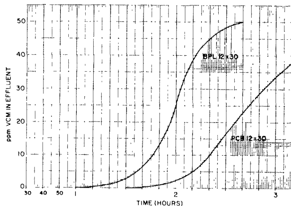
FIGURE 3 - 50 ppm VINYL CHLORIDE IN AIR
