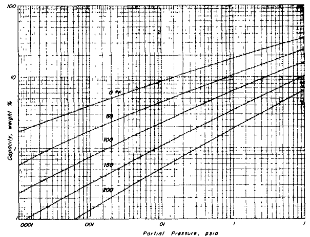
FIGURE 6 - ADSORPTION OF VINYL CHLORIDE ON BPL
