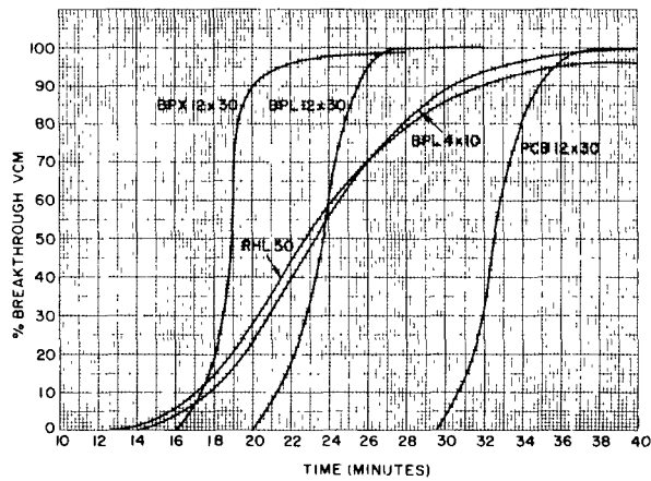
FIGURE 2 - 1% VINYL CHLORIDE IN AIR
