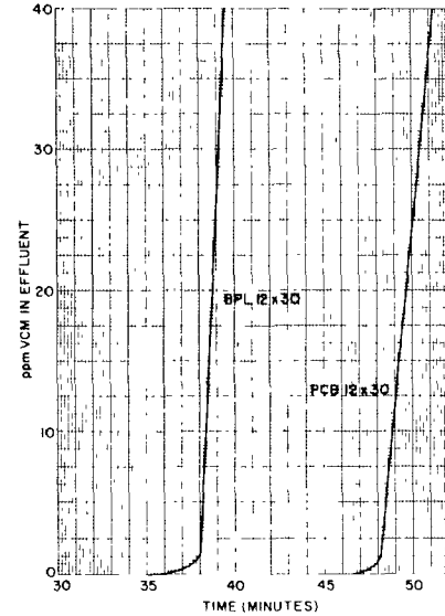
FIGURE 4 - 1% VINYL CHLORIDE IN AIR
