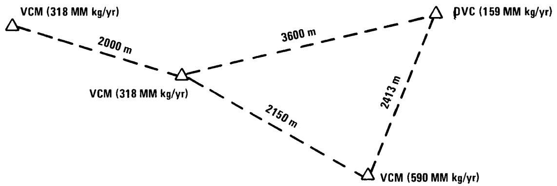
Figure 6-2. Map of four plant cluster - Case II.
