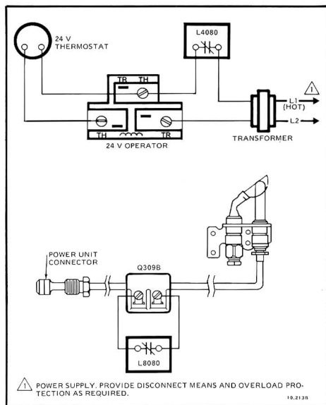
Fig. 3—Typical wiring hookup for 24 V systems.
