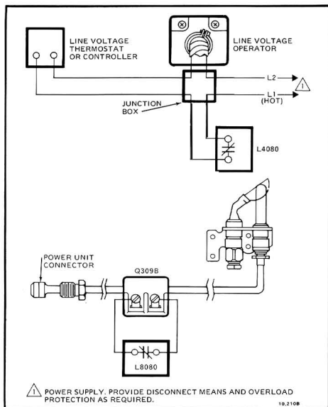
Fig. 4—Typical wiring hookup for line voltage system.
