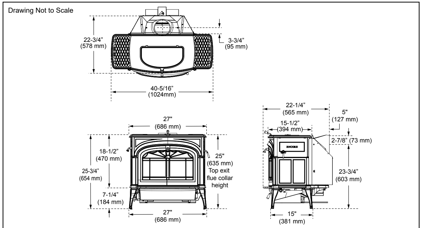
Figure 1 - Encore® 2040 dimensions.
