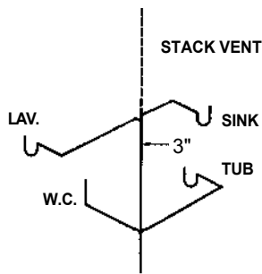
Stack Venting Figure 9-37
