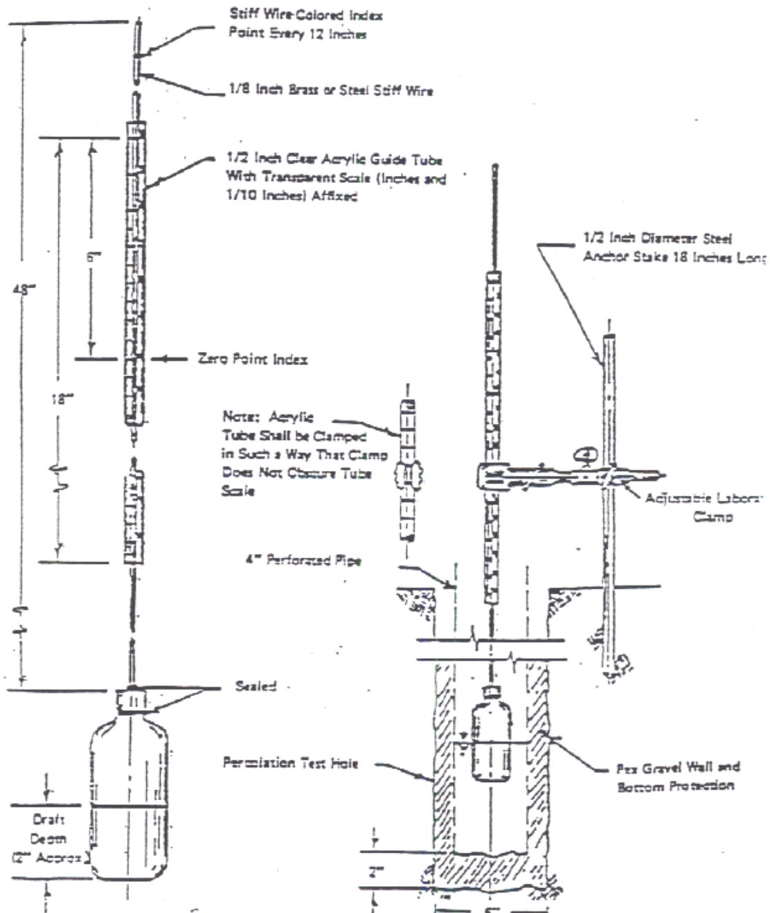
FLOAT GAUGE AND PERCOLATION TEST ASSEMBLY Reference Section 20.06.06 A
