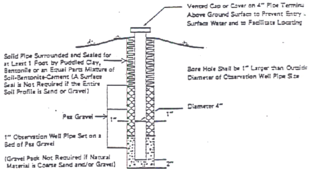
Diagram D2 Monitoring Well Design Reference Section 20.06.09 C
