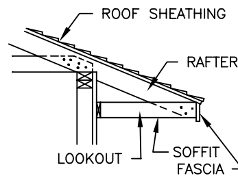
EAVE OVERHANG (RAFTER)
