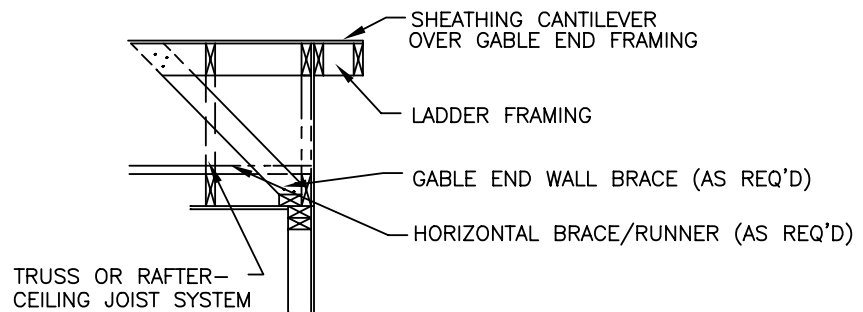
RAKE OVERHANG (LADDER)
