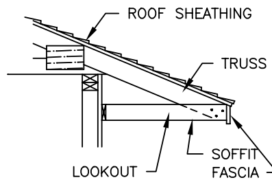
EAVE OVERHANG (TRUSS)
