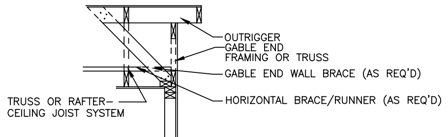
RAKE OVERHANG (OUTRIGGER)
