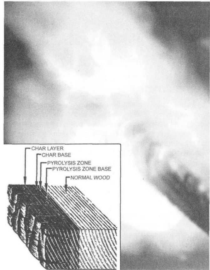
Figure 6.2 Degradation zones in a charred piece of wood [8]
