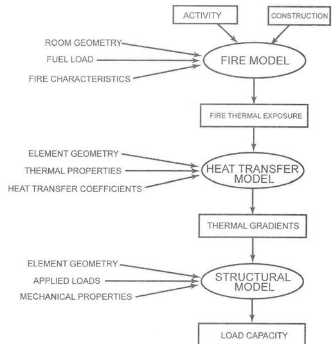
Figure 6.1 A fire-damaged building at the US Forest Products Laboratory and a flowchart [1] for modeling fire-damaged wood members in a structural fire
